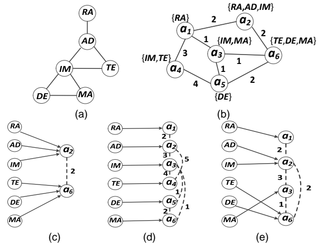
Fig. 1. A simple complex task allocation example in a social network. (a) the complex task P=\{RA, AD, IM, TE, DE, MA\} ; (b) the social network; (c) task allocation Scheme 1 of satisfying P 's skill requirements (the arrow represents the task allocation and the dash line represents the necessary communication and the number attached to each dash line represents its communication cost); (d) task allocation Scheme 2 of alleviating employers' workloads; (e) task allocation Scheme 3 of improving employers' communication efficiency.
