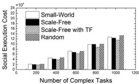
Fig. 7. The effect of the network properties on social execution cost.
