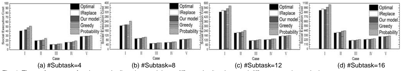
Fig. 4. The performance of various task allocation models on different (\alpha, \beta) values and different complex task sizes.
