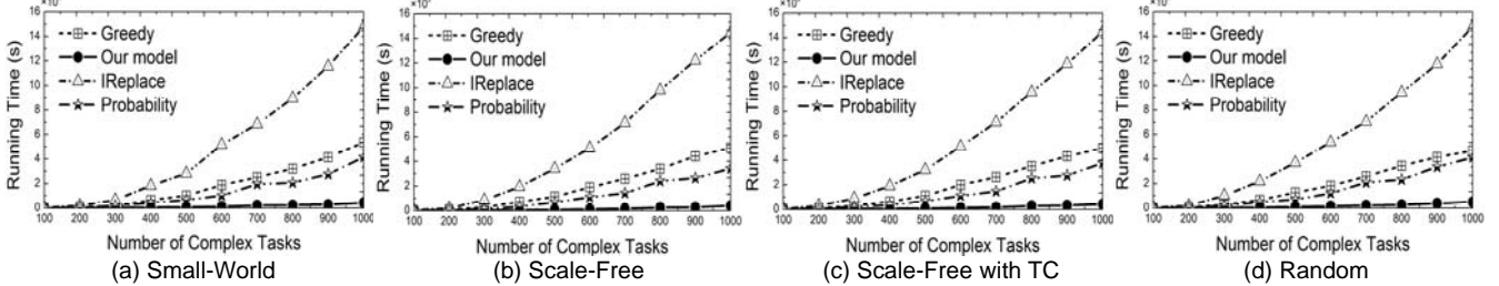
Fig. 6. The running times of different models in the large-scale applications.
