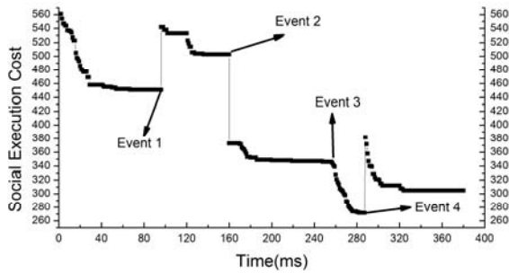
Fig. 8. The social execution cost plot with four disturbance events.
