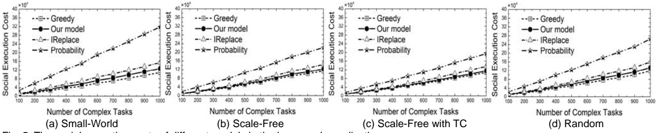
Fig. 5. The social execution costs of different models in the large-scale applications.
