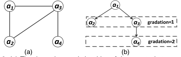
Fig. 3. (a) The dependency relationships of the agents that queue at node n_2 . (b) The negotiation process of agent a_1 .
