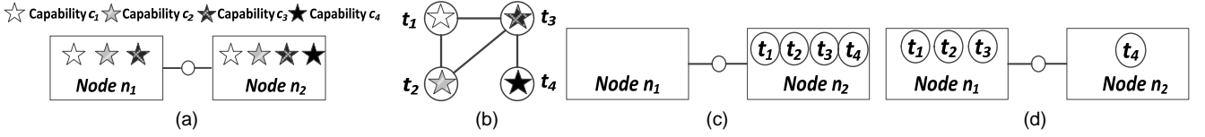
Fig. 2. A simple social complex task allocation instance. (a) The network. (b) The complex task. (c) The equilibrium solution S=\{n_2, n_2, n_2, n_2\} . (d) The optimal solution S^*=\{n_1, n_1, n_1, n_2\} .
